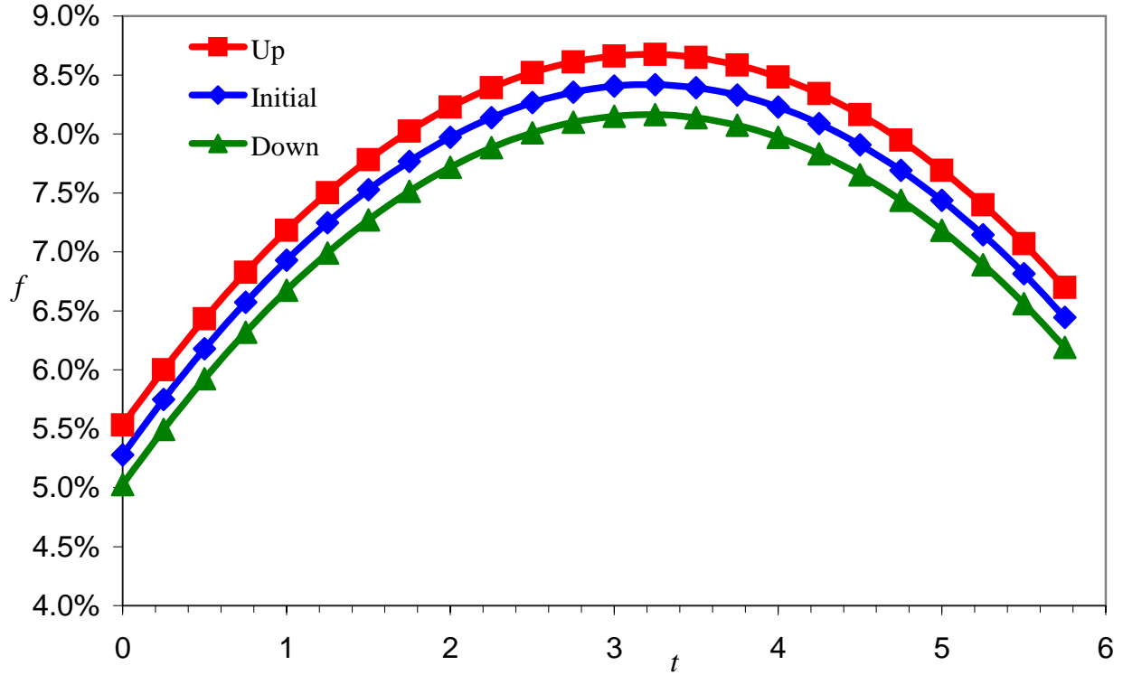
Figure 2: Yield curves (rigid shift)
